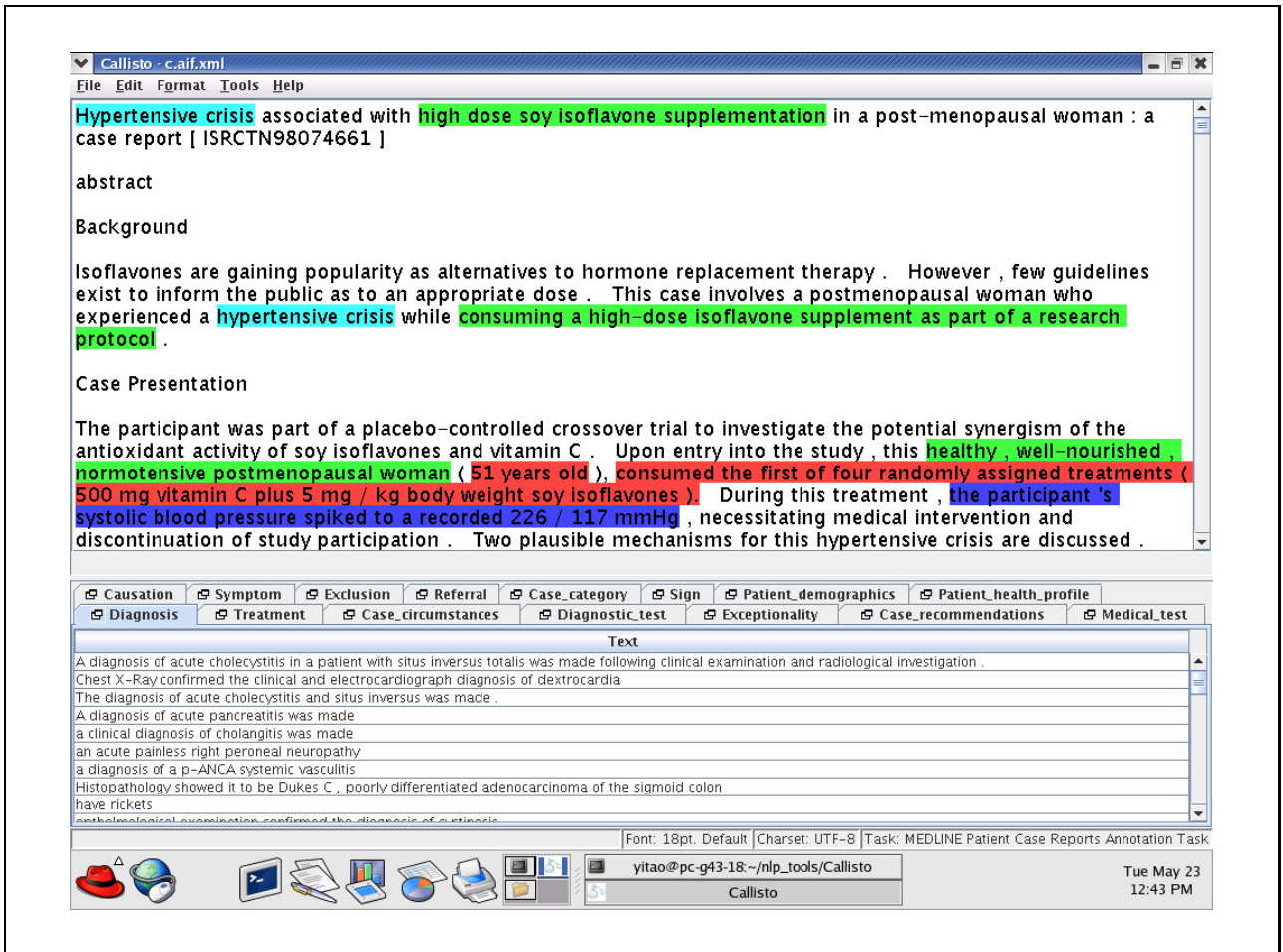
Figure 1: The Callisto GUI for Manual Annotations
