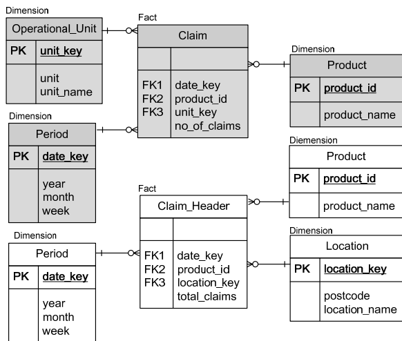
Figure 1: Star Schema
