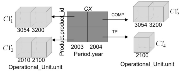
Figure 4: Drill Across from a Common Data Space to C1
