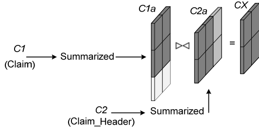
Figure 3: Obtaining of the common data space
