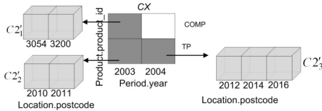
Figure 5: Drill Across from a common data space to C2
