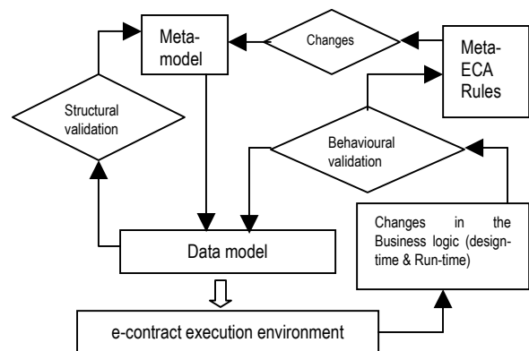
Figure 1: Active meta-modeling of e-contracts
