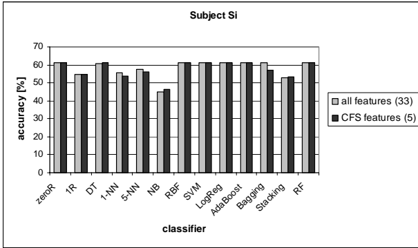
Figure 5: Off-line evaluation of the classifiers built for the pong game. Accuracy [%] using 10-fold cross-validation for subject Si
